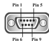
RS232 Pinout (9 Pin Male)
